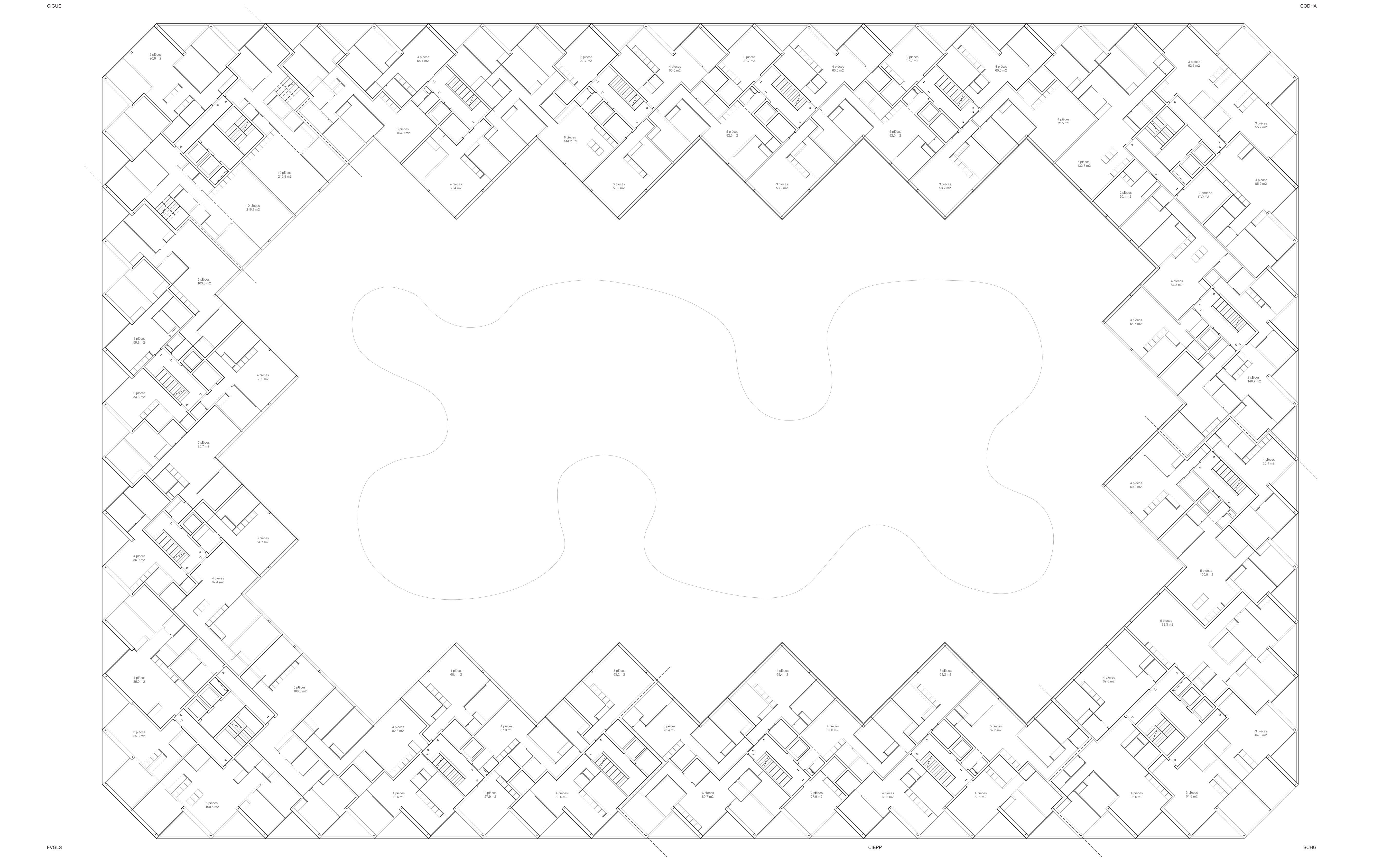
PLAN ETAGE TYPE ILOT A 1:200
