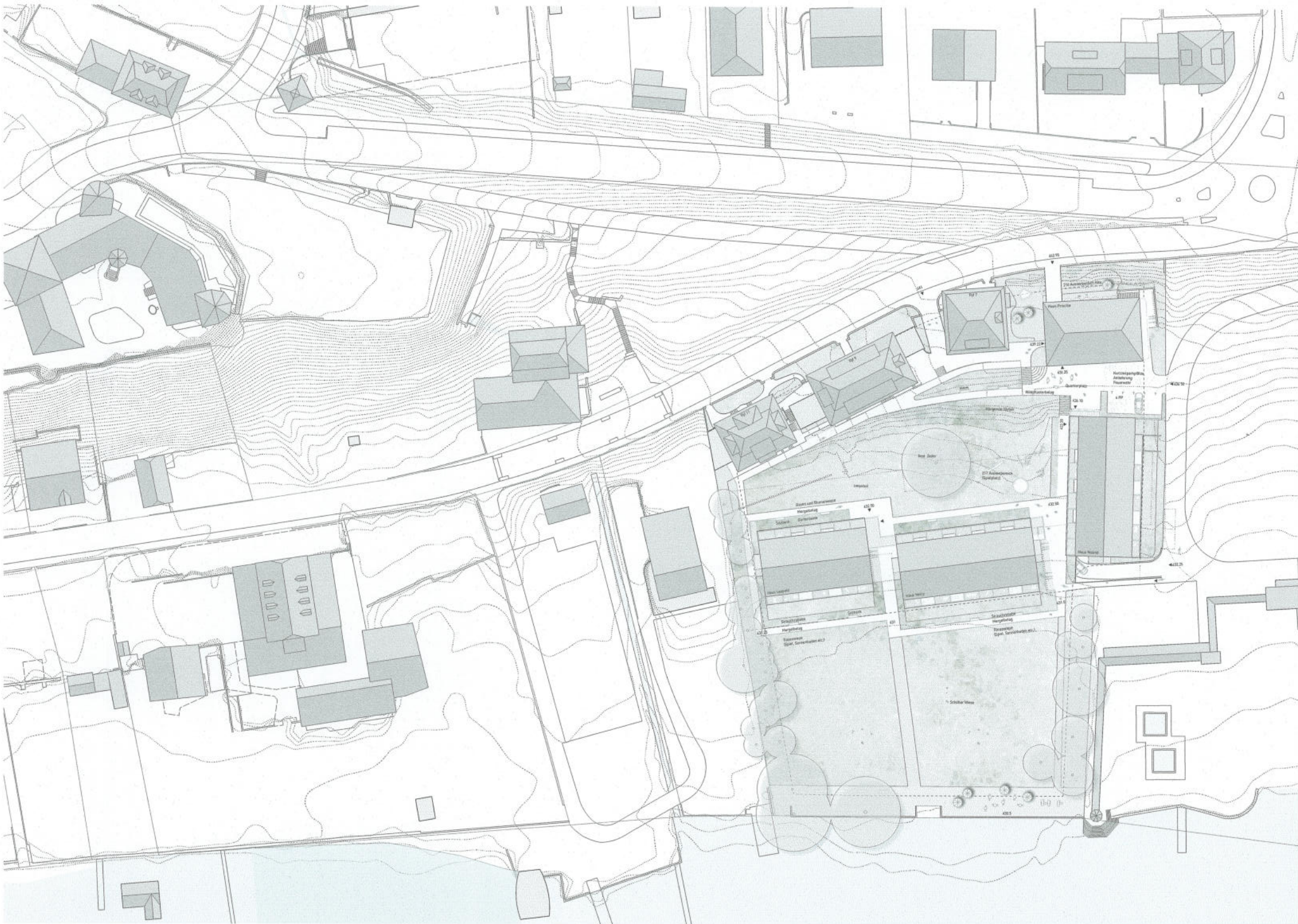
Situationsplan 1:500
