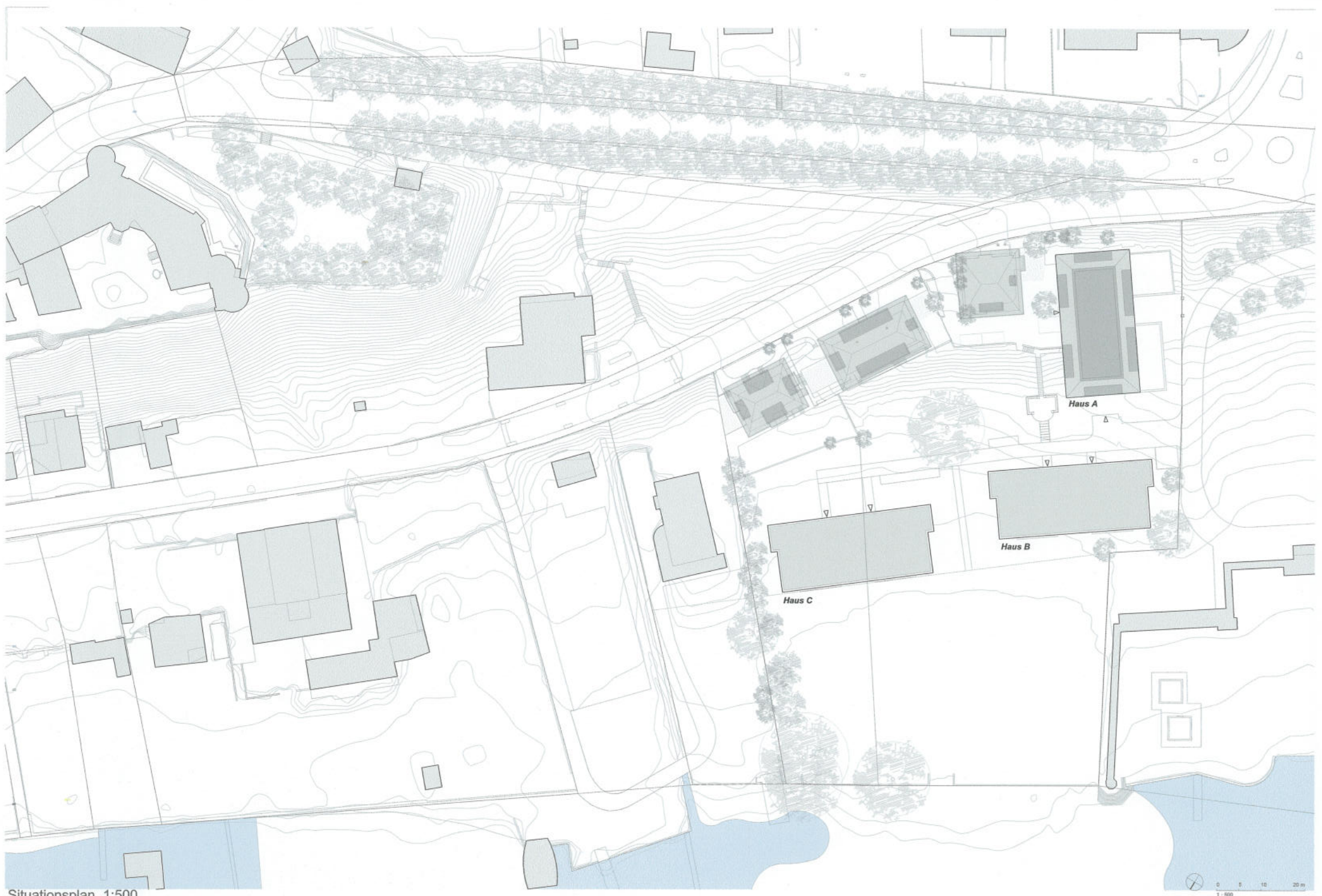
Situationsplan 1:500
