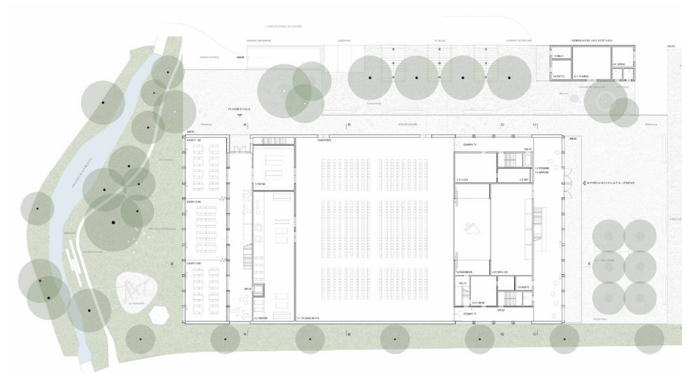
Erdgeschoss MZH
