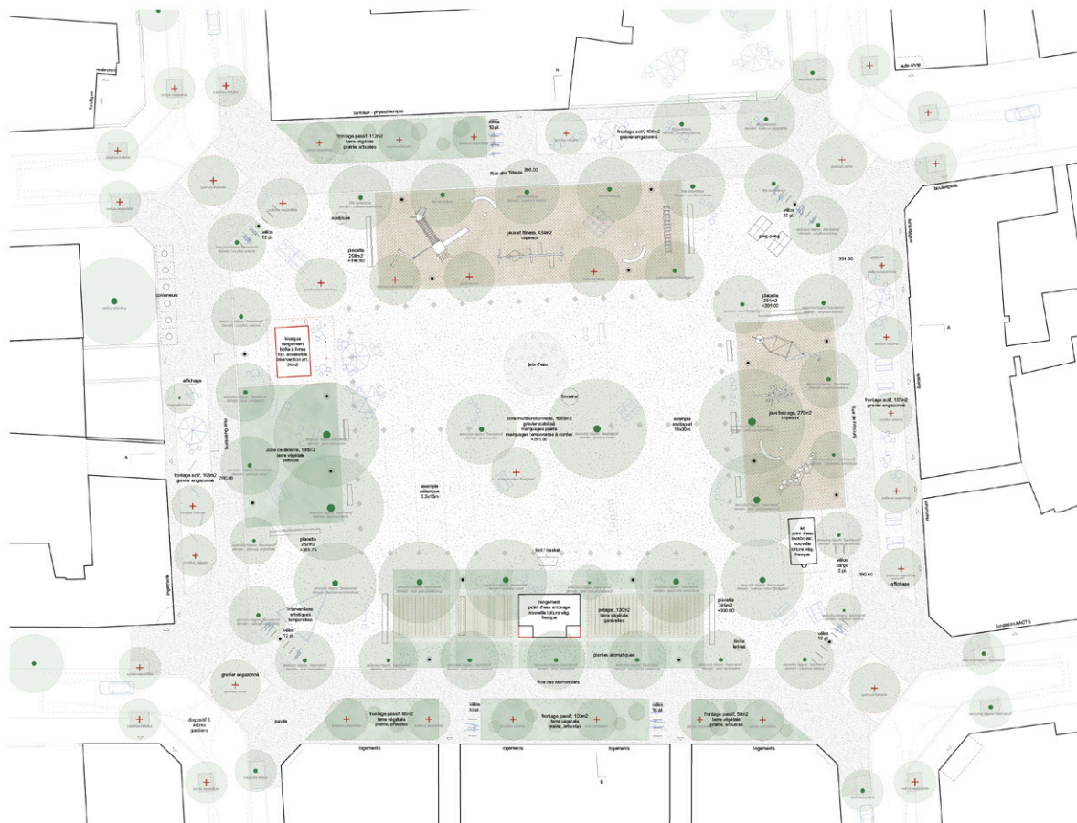
Plan 1:200
