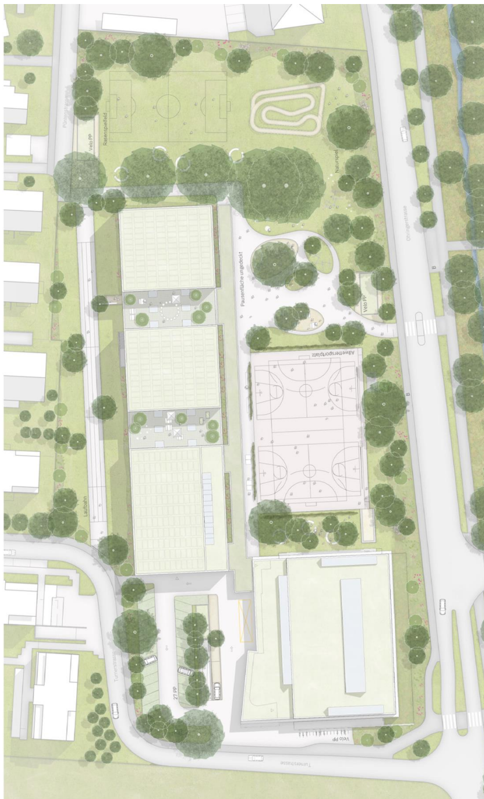
Abb. 51 Situation
