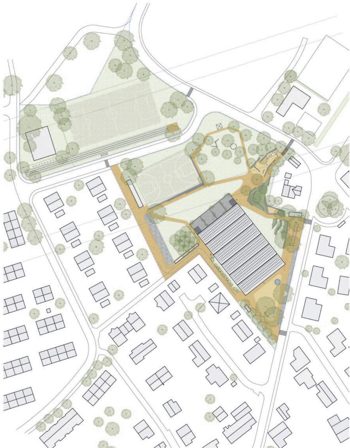
Situation 1:1500
