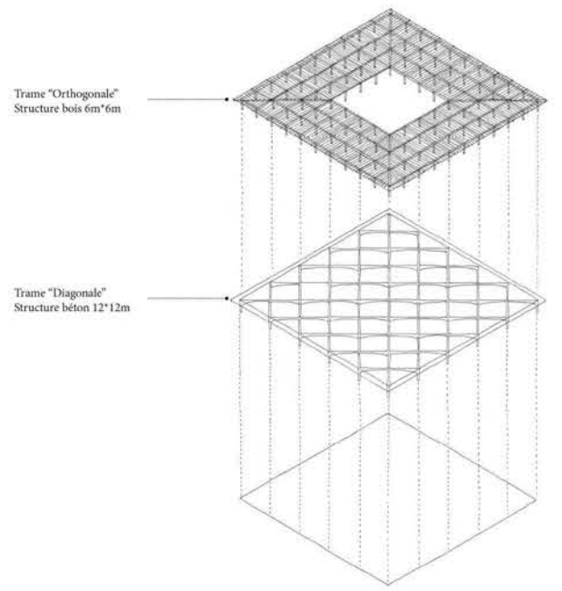
Concept structurel
