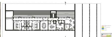
PLAN R+1 1:200
