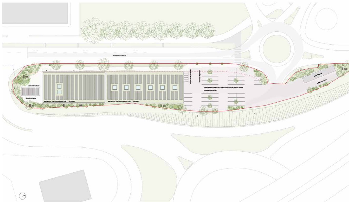
Situationsplan 1:500 10 15 110 | 25
