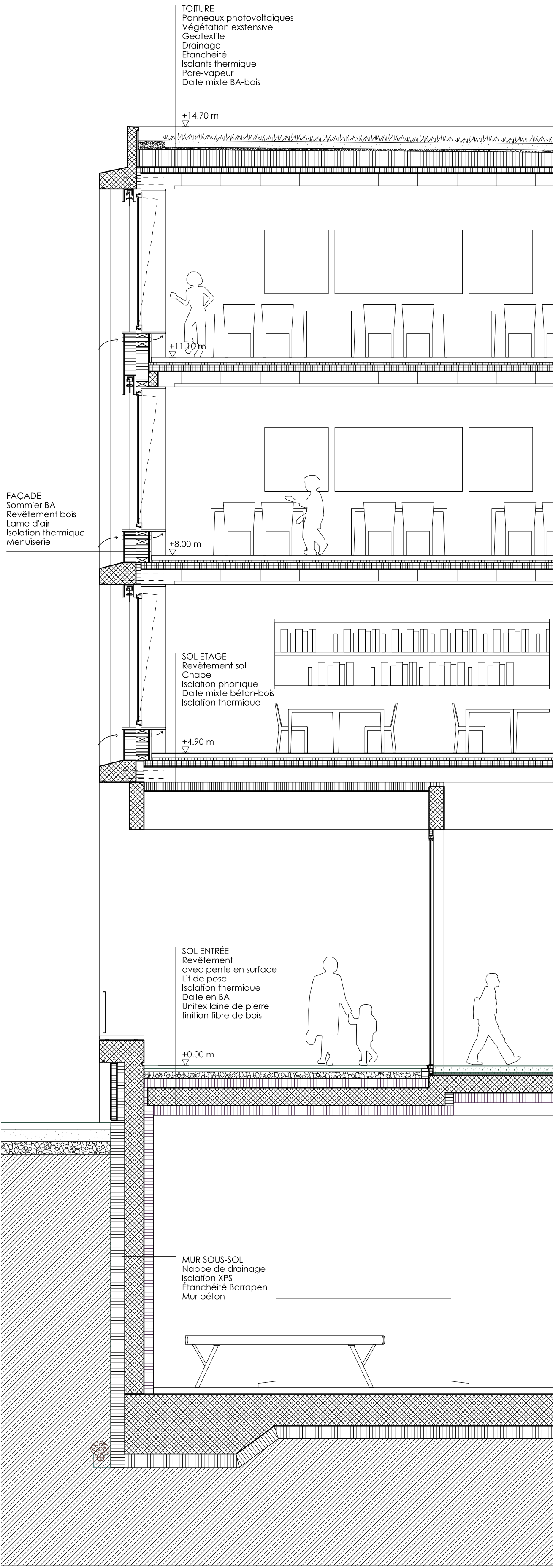
Coupe constructive - 1/50
