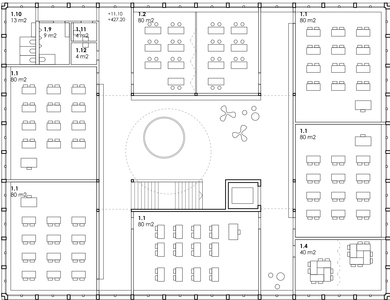
Plan R+3 - 1/200
