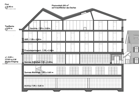
Querschnitt (Ost-West)
