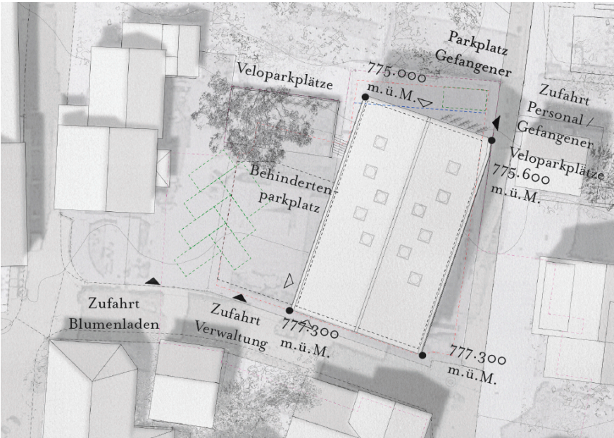
Situation
