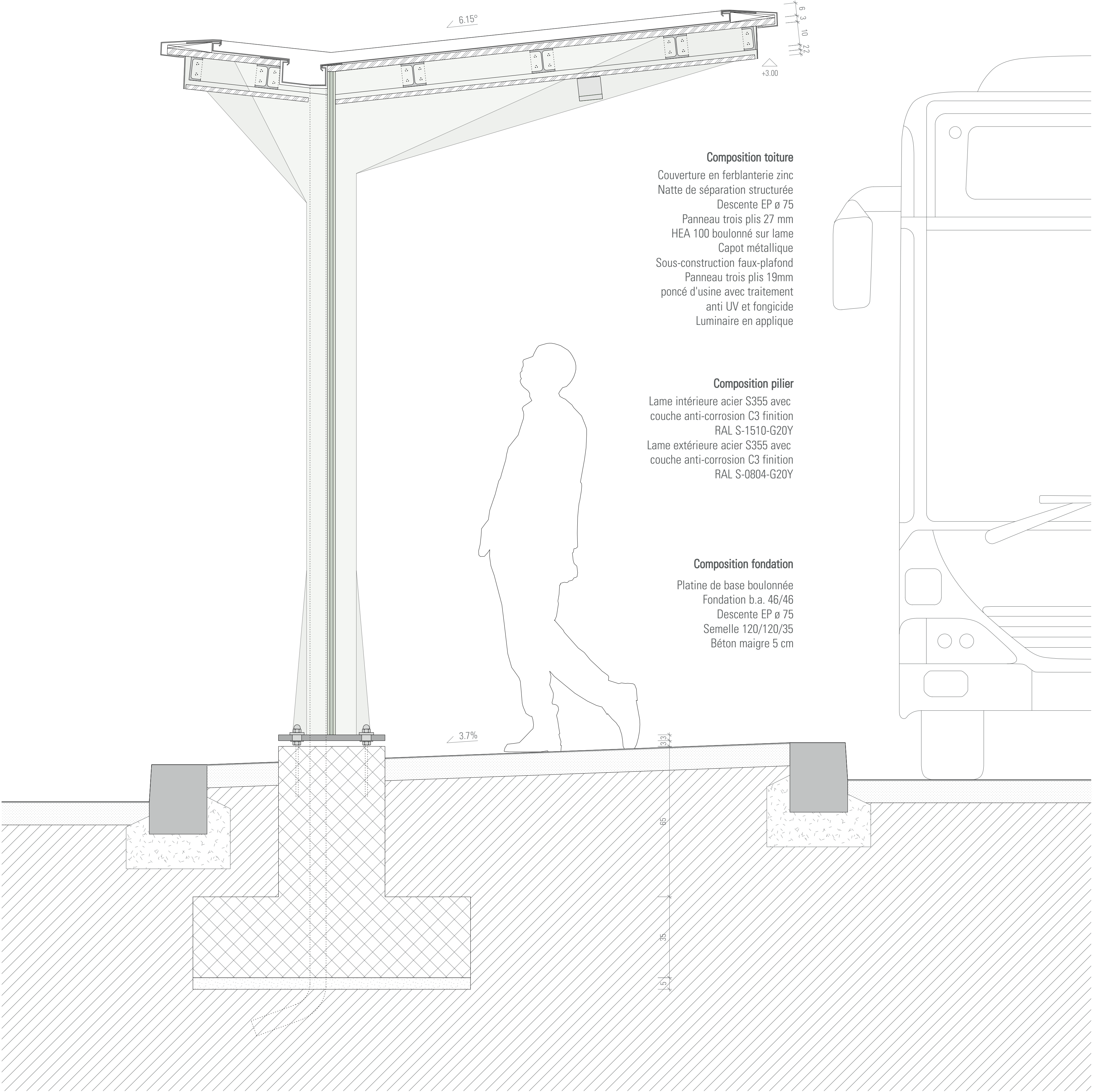
DETAIL 1:10
