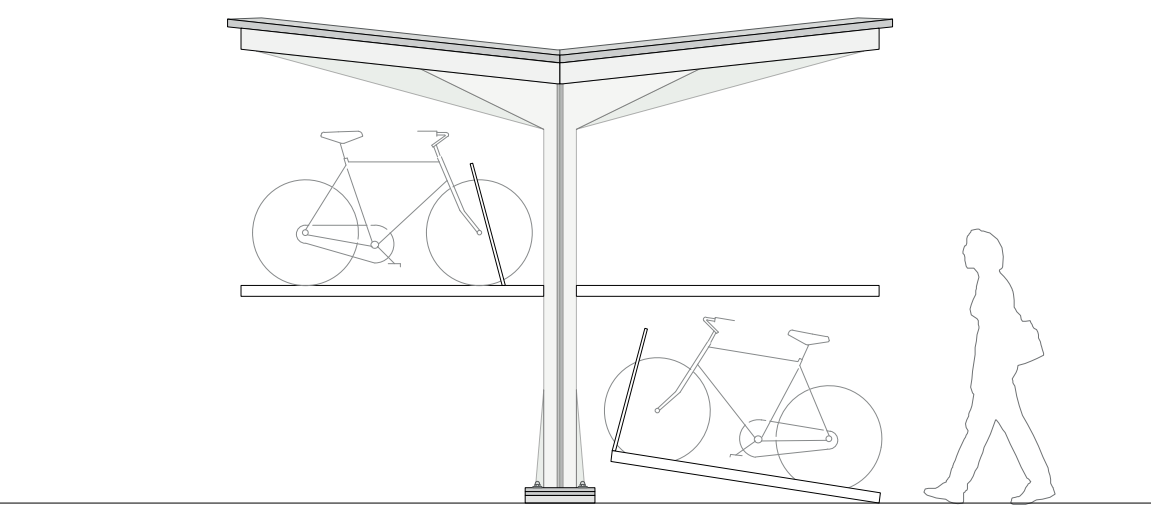
PERIMETRE IV COUVERT A VELO 1:50
