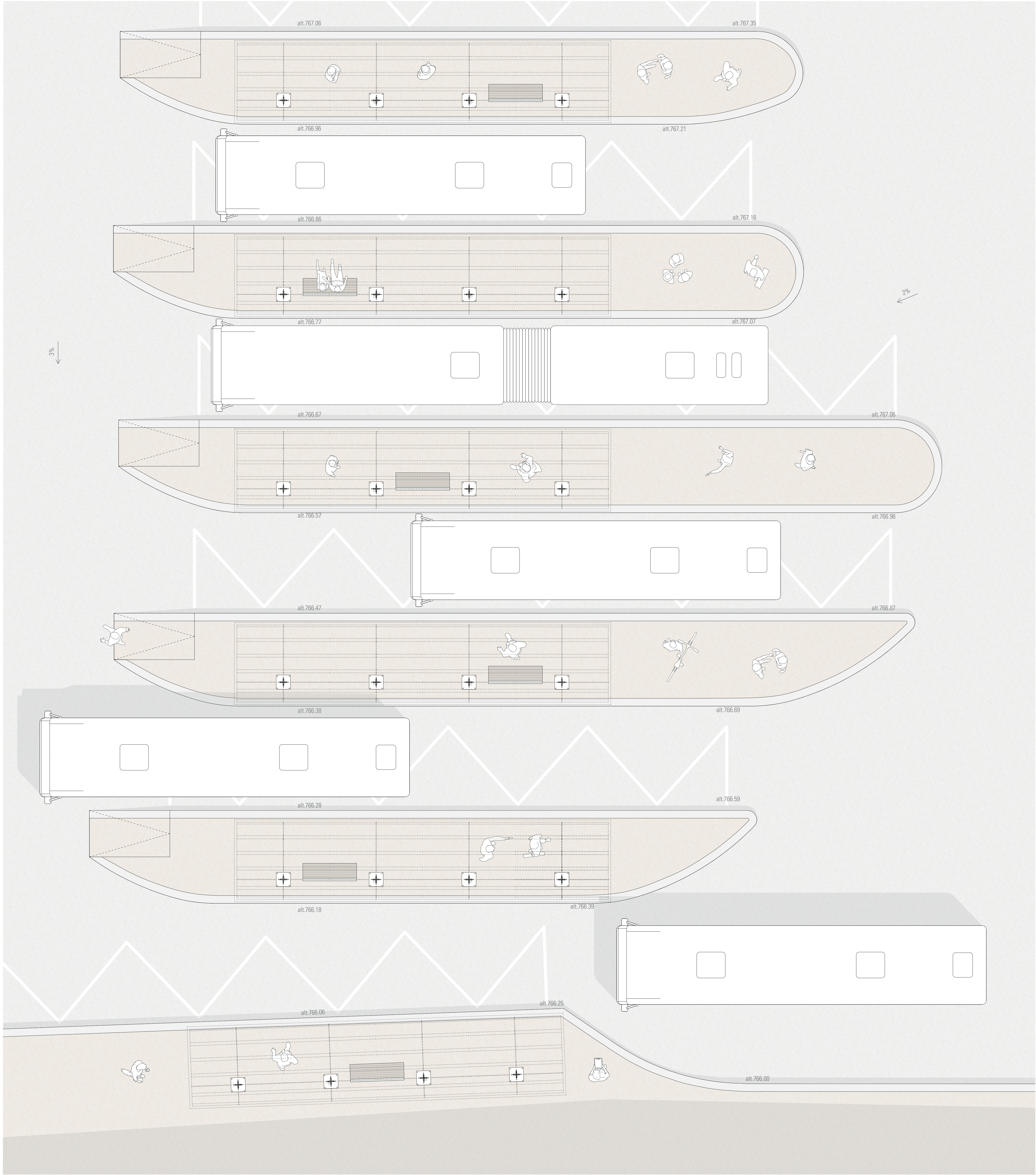
PLAN PERIMETRE | BUS REGIONAUX 1:50
