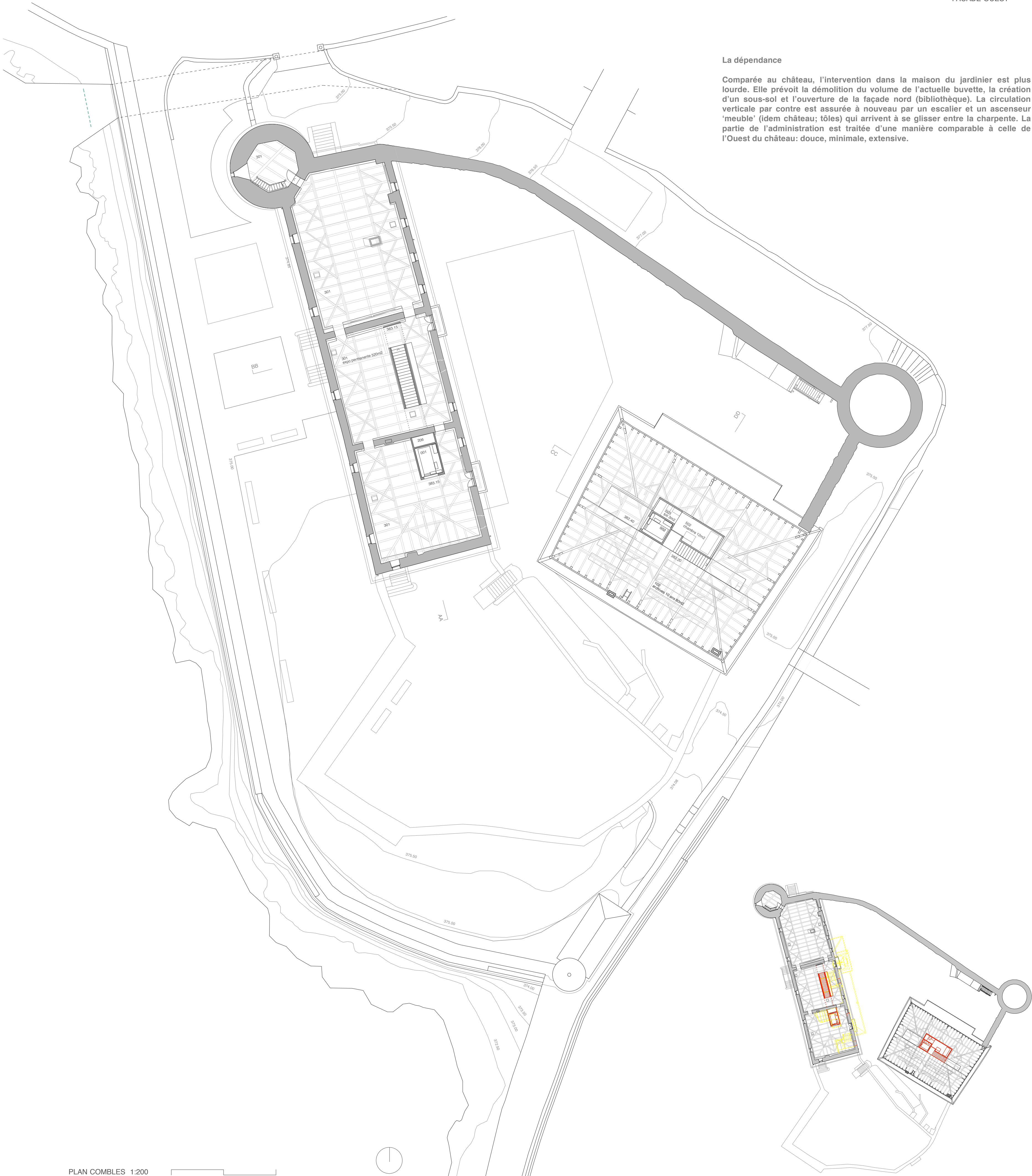
PLAN COMBLES 1:200
