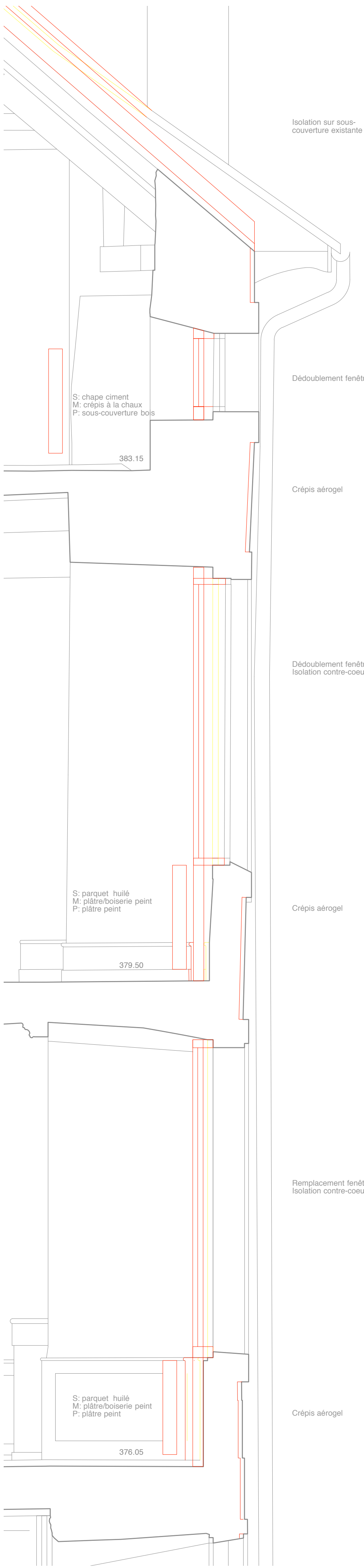
COUPE FACADE 'CHATEAU' 1:20
