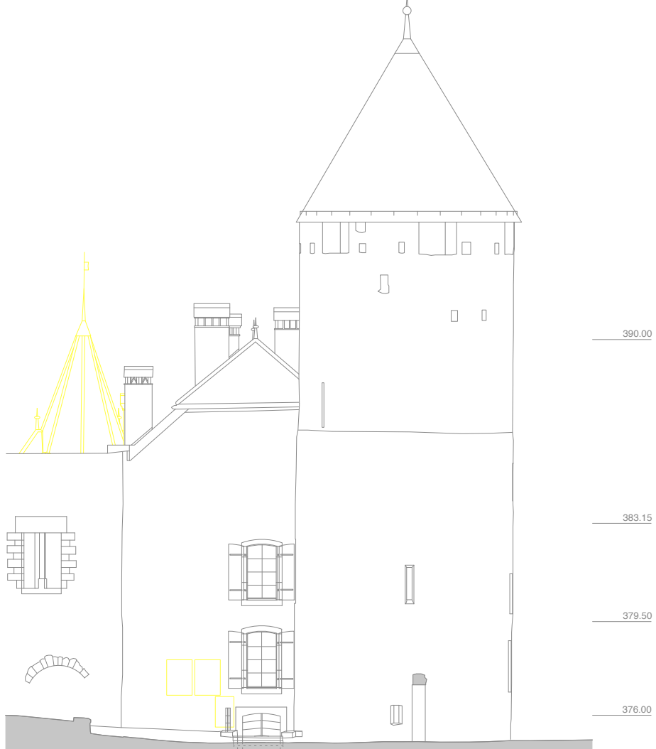
FACADE SUD
